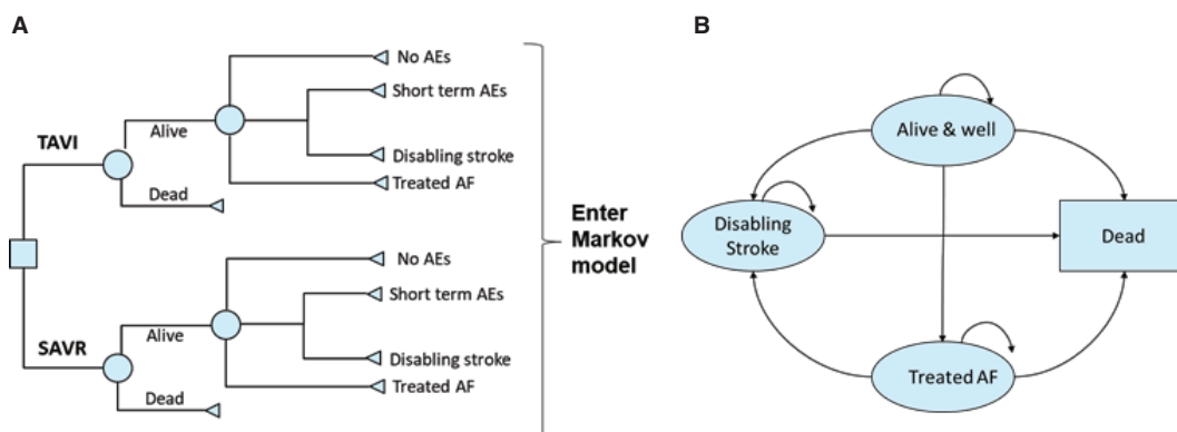
Figure 1. The cost-effectiveness model had two stages: (A) early AEs from the PARTNER 3 trial were captured in a decision tree, which fed into (B) a Markov model that captured longer-term outcomes of patients, with four distinct health states. a
